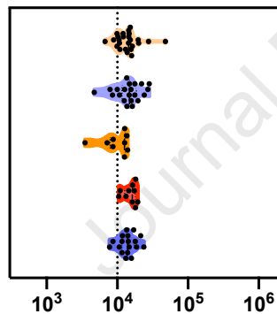
NL63-RBD
