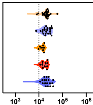
229E-RBD
