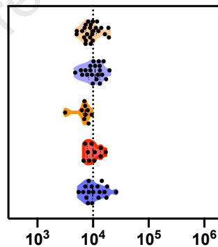
HKU1-RBD
