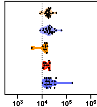
OC43-RBD
